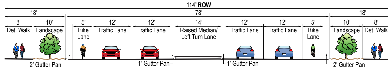
Four-Lane Urban or Semi-Urban Arterial
