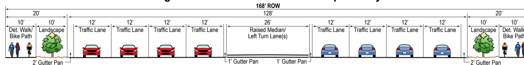
Eight-Lane Urban or Semi-Urban Expressway
