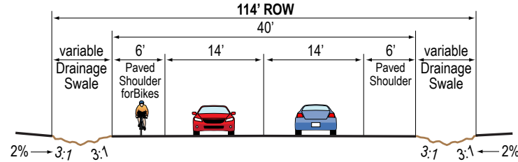
Two-Lane Rural Arterial with or without Bike Accommodations
