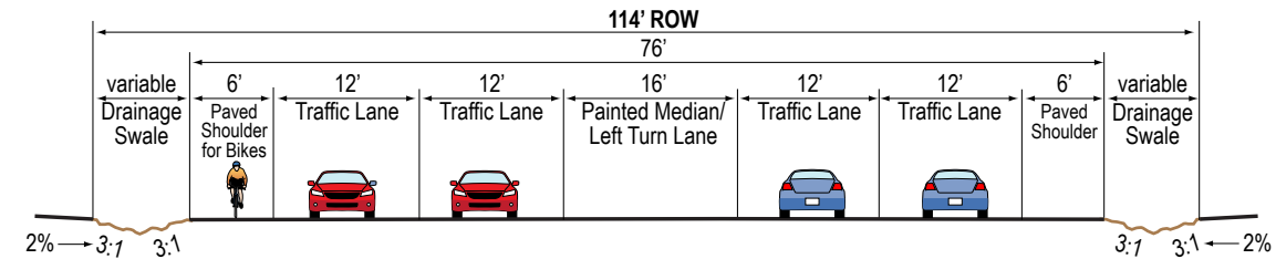
Four-Lane Rural Arterial
