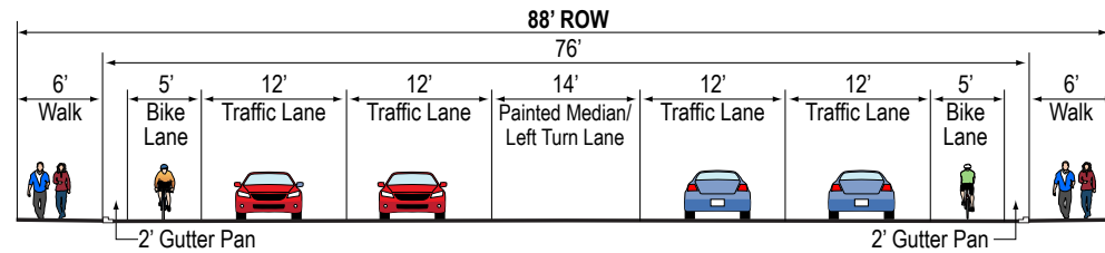
Four-Lane Urban or Semi-Urban Collector
