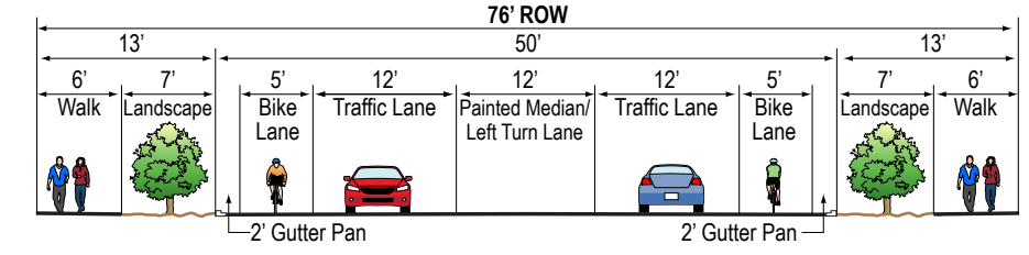
Two-Lane Urban or Semi-Urban Collector
