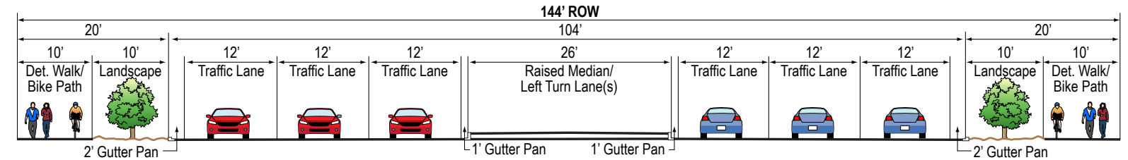
Six-Lane Urban or Semi-Urban Arterial
