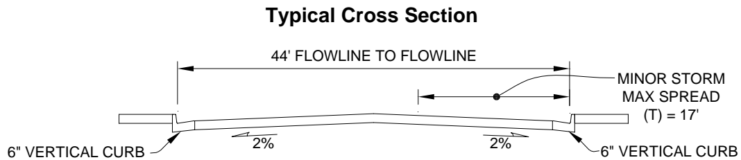
FIGURE 7-15, ARAPAHOE COUNTY STREET CAPACITY CHART 60' MINOR COLLECTOR (1986 MANUAL)
