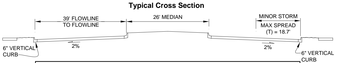
FIGURE 7-19, ARAPAHOE COUNTY STREET CAPACITY CHART 140' (6 LANE) MAJOR ARTERIAL (1986 MANUAL)
