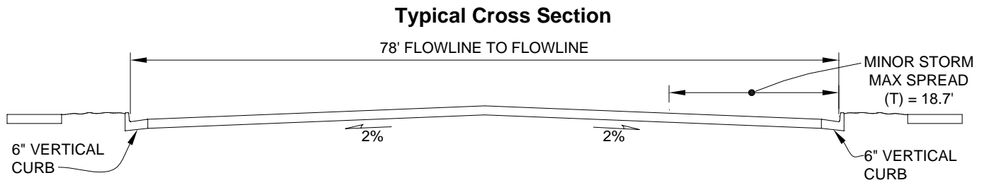
FIGURE 7-9, ARAPAHOE COUNTY STREET CAPACITY CHART FOUR-LANE ARTERIAL WITH PAINTED MEDIAN
