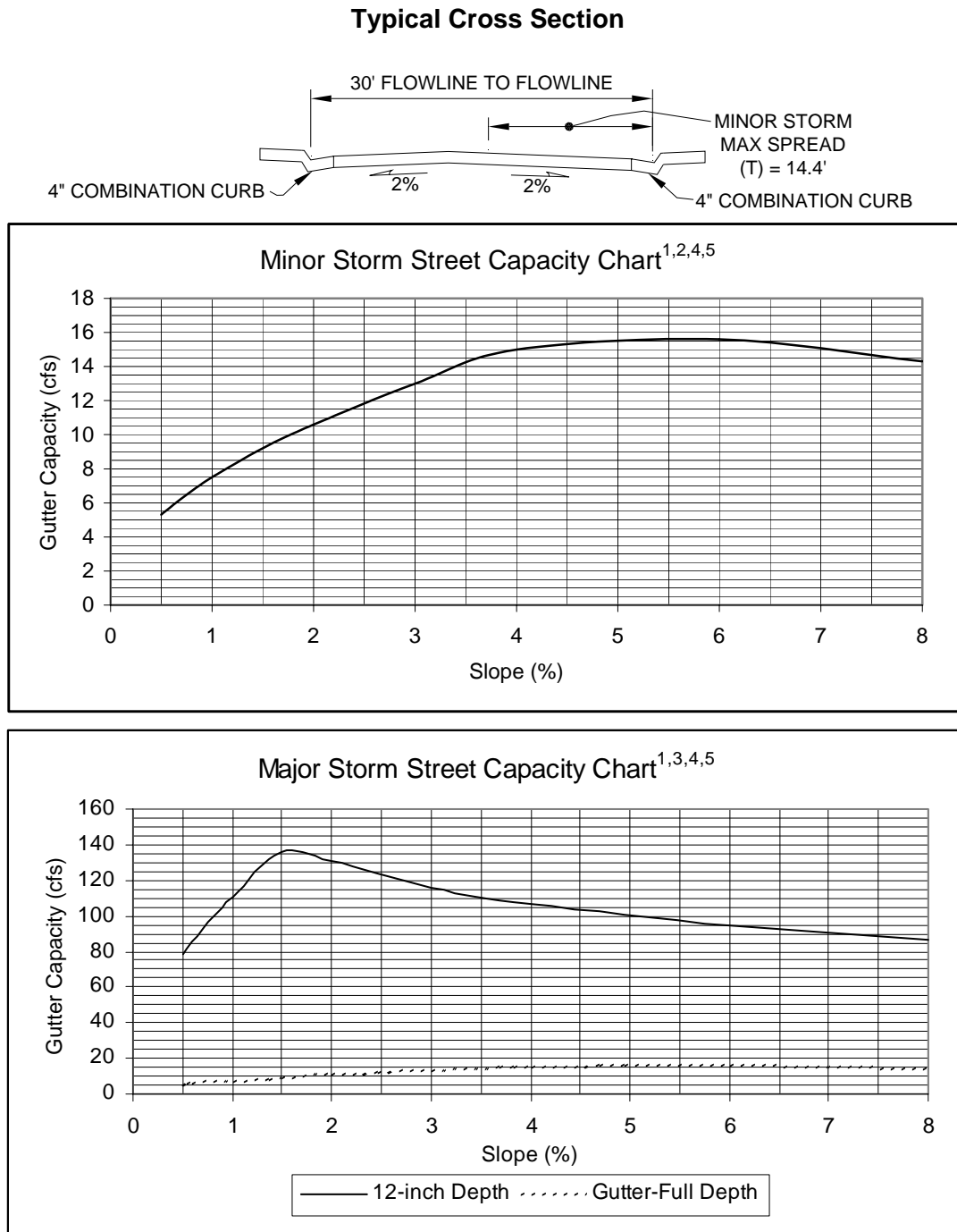
FIGURE 7-1, ARAPAHOE COUNTY STREET CAPACITY CHART URBAN PRIVATE – PARKING ONE SIDE (4" CURB)
