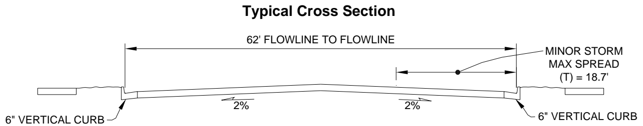
FIGURE 7-8, ARAPAHOE COUNTY STREET CAPACITY CHART FOUR-LANE COLLECTOR
