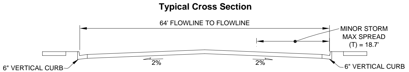
FIGURE 7-17, ARAPAHOE COUNTY STREET CAPACITY CHART 100' MINOR ARTERIAL (1986 MANUAL)
