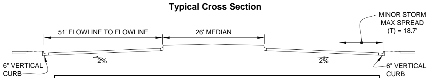
FIGURE 7-12, ARAPAHOE COUNTY STREET CAPACITY CHART EIGHT-LANE URBAN EXPRESSWAY
