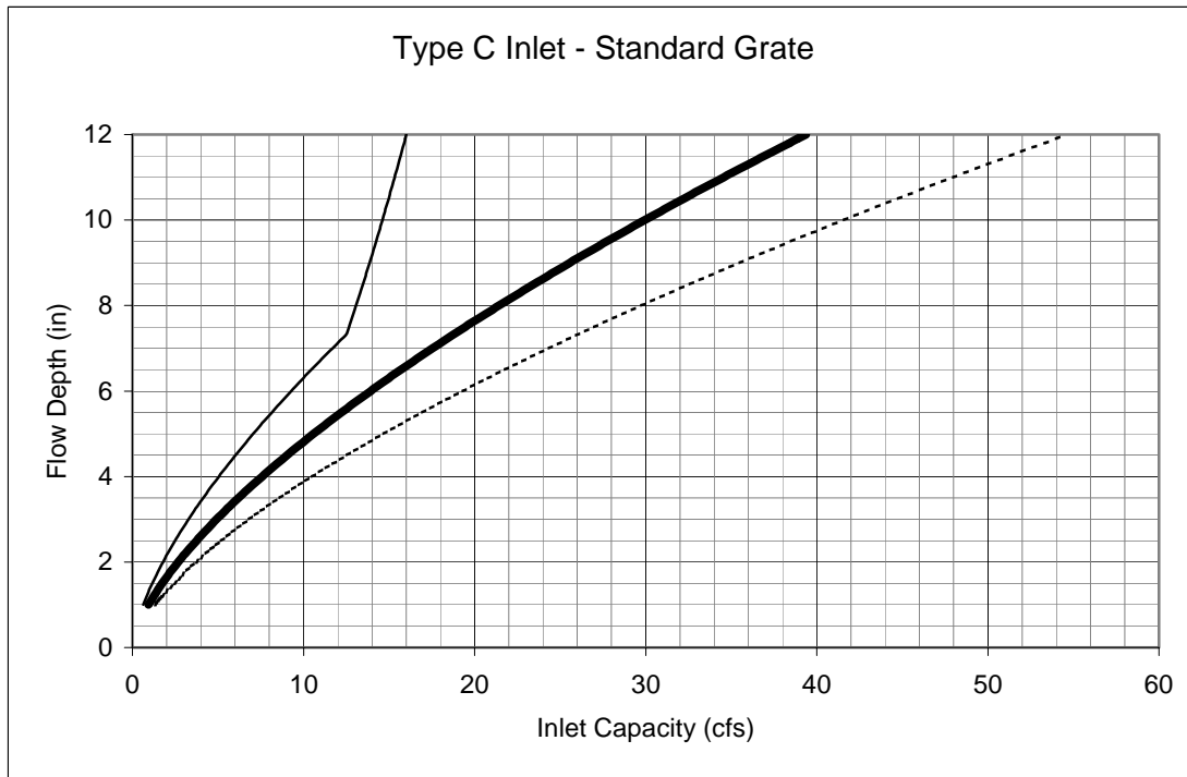
FIGURE 8-21, INLET CAPACITY CHART SUMP CONDITIONS AREA (TYPE C) INLET
