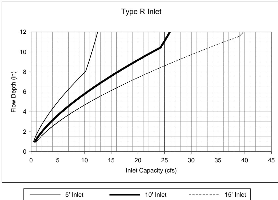
FIGURE 8-22, INLET CAPACITY CHART SUMP CONDITIONS CURB OPENING (TYPE R) INLET
